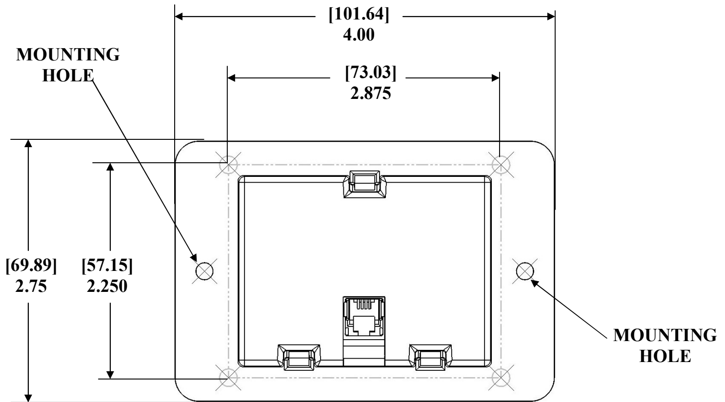
Figure 5 PD1201 Remote Display Mounting Template
