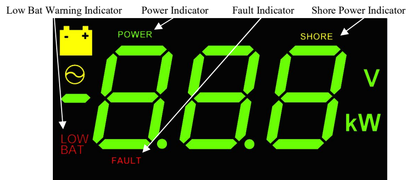
Figure 5 Display Indicators
